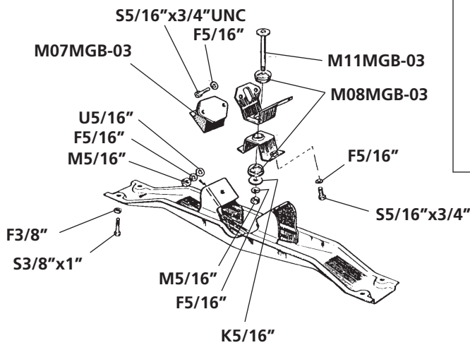
Type 2 (65-67) 3-Synchro GT
