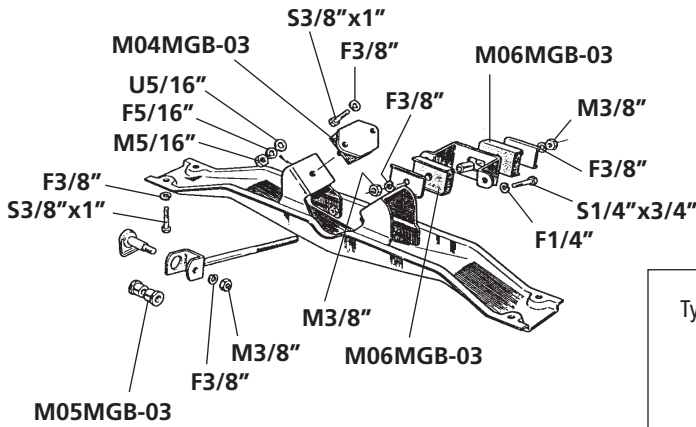
Type 1 (62-67) 3-Synchro Roadster
