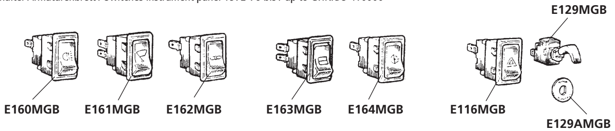
Schalter Armaturenbrett / Switches instrument panel ab / from 1976 ab / from GHN/D5 410001
